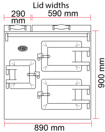
EVH 90 Plus right-hand oven front view
