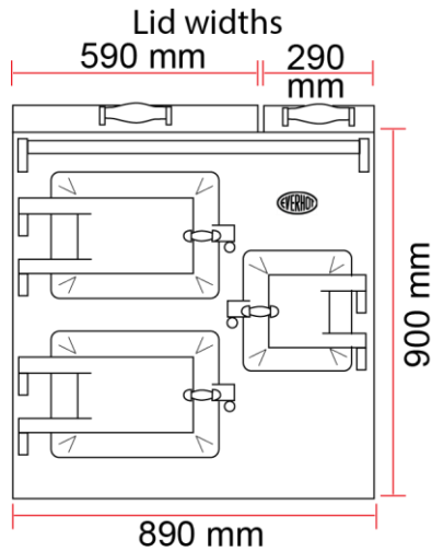
EVH 90 Plus left-hand oven front view
