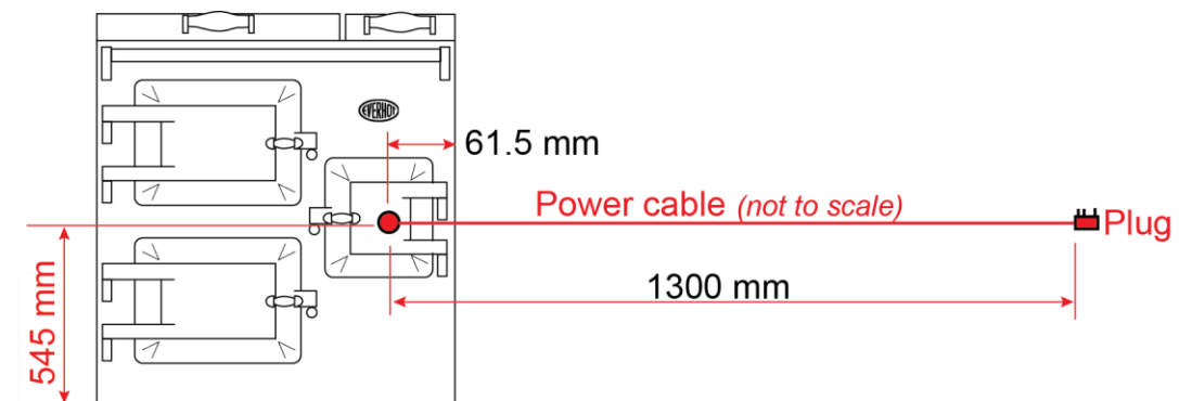
EVH 90 Plus left-hand oven cable lengths
