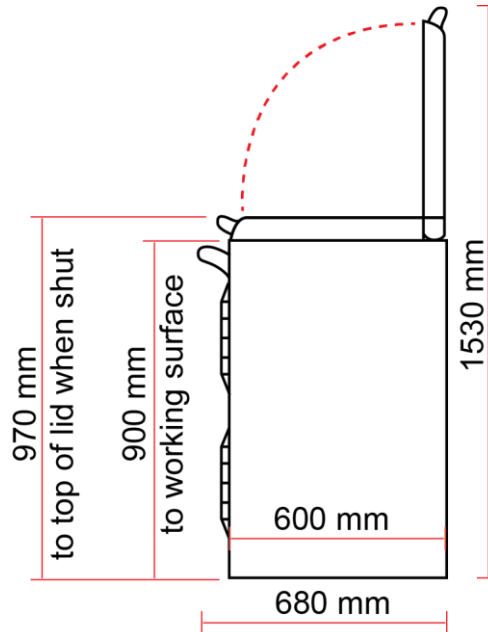
EVH 90 Plus side view
