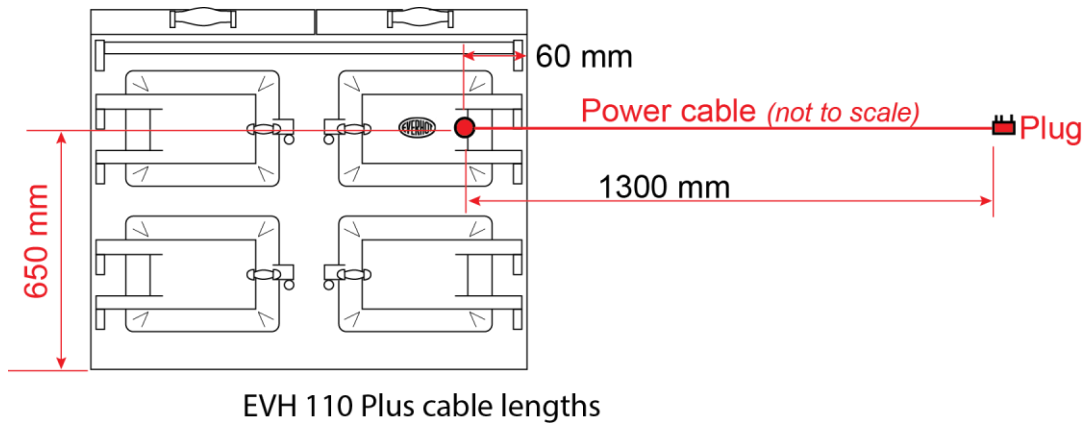
EVH110+ dimensions
