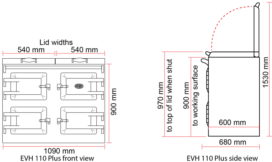
EVH110+ dimensions
