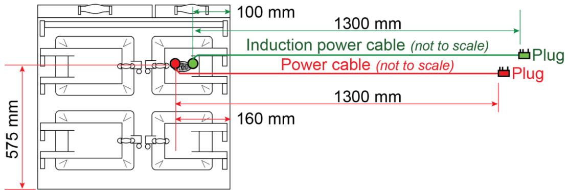
EVH100i cable lengths
