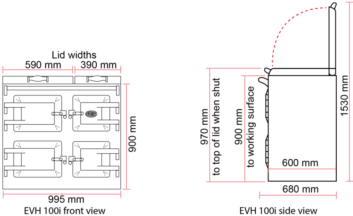
EVH100i dimensions
