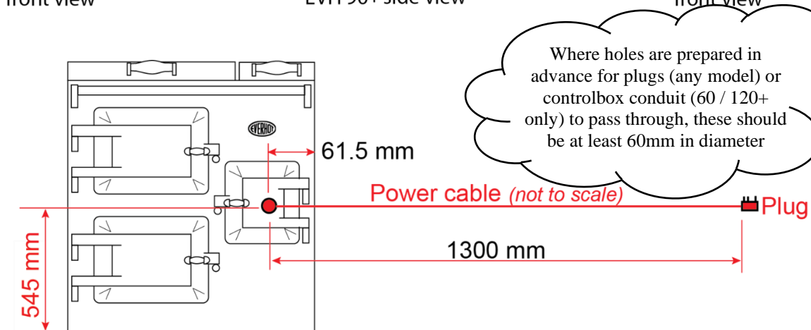
EVH 90+ left-hand oven cable lengths
