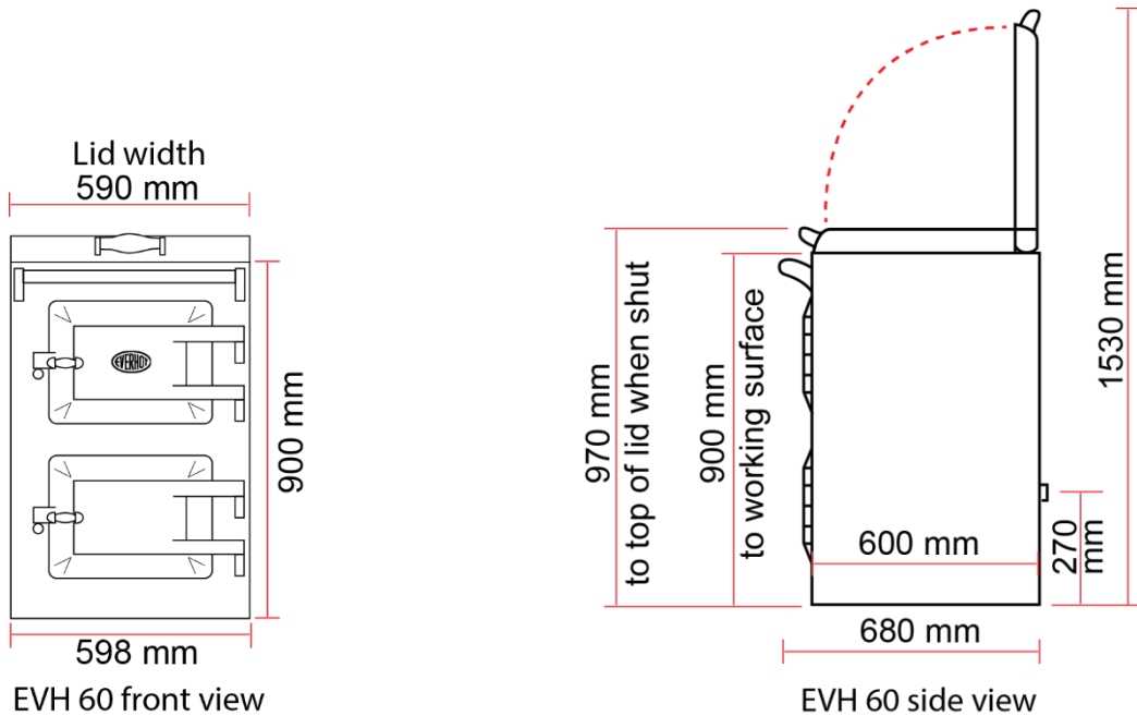
EVH60 dimensions
