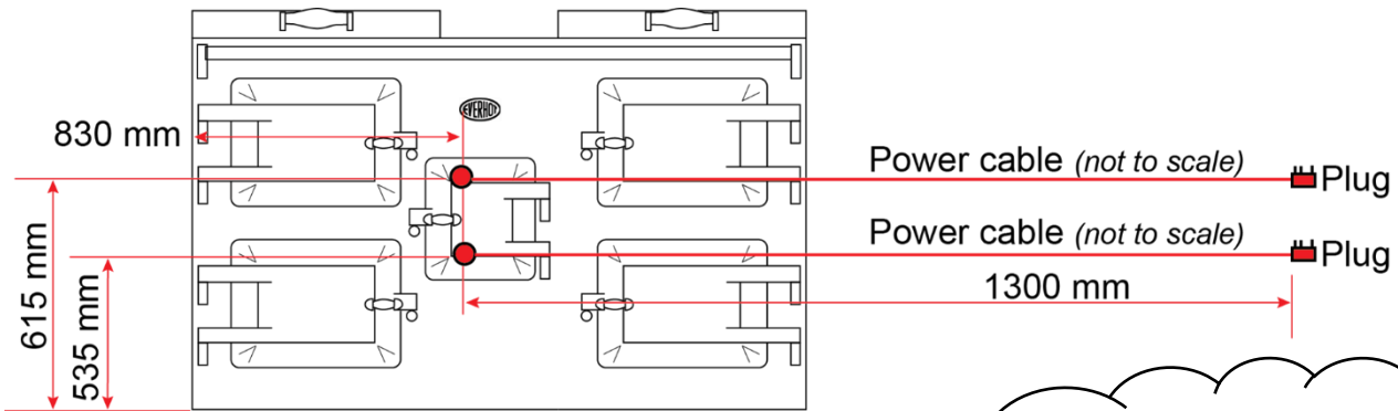
EVH 150+ cable lengths
