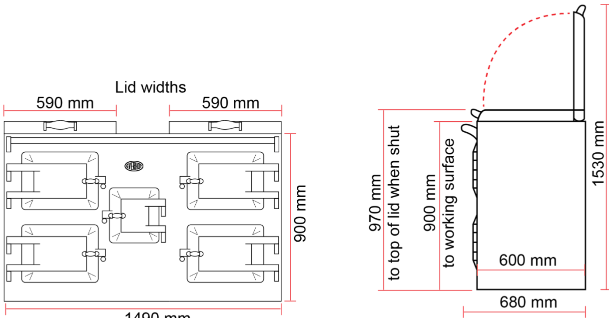
EVH 150+ front view
