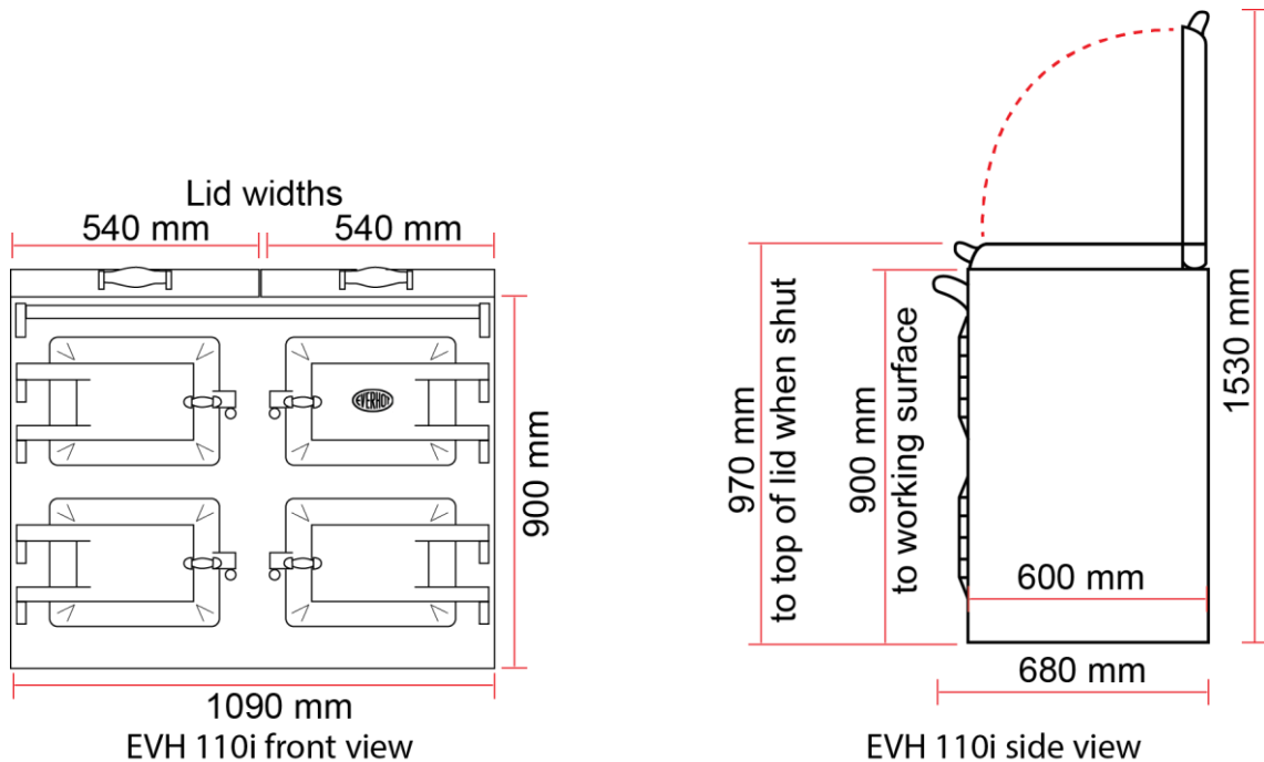
EVH110i dimensions
